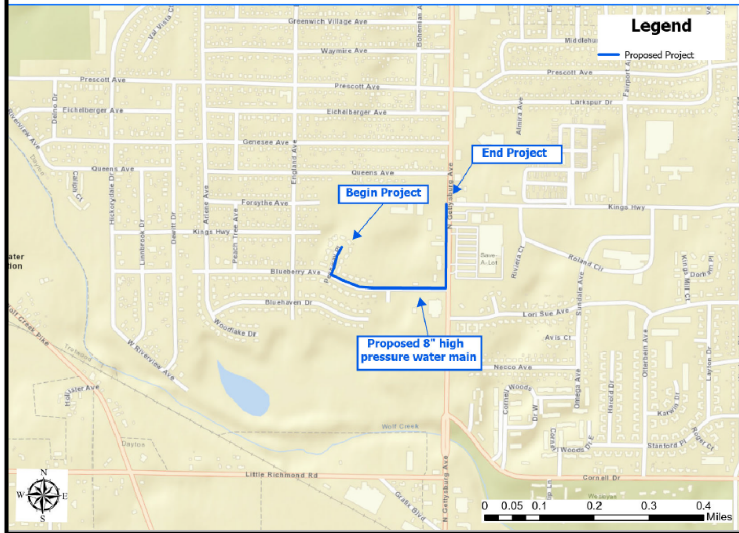
Figure 2-Gettysburg-Blueberry-Pennway Water Main Improvements Project Limits
